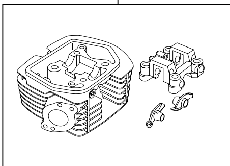
01-03-0775 Super Head ST-3 Head Kit
